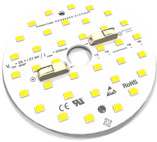
Downlight
